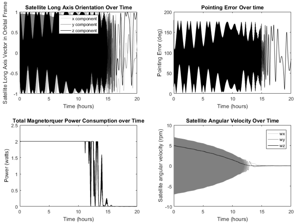
Figure 14: B-Dot Only in 700 km Circular Orbit
