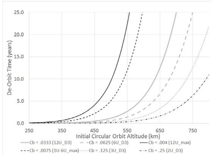
Figure 12: Orbit Lifetime vs. Initial Circular Orbit Altitude
