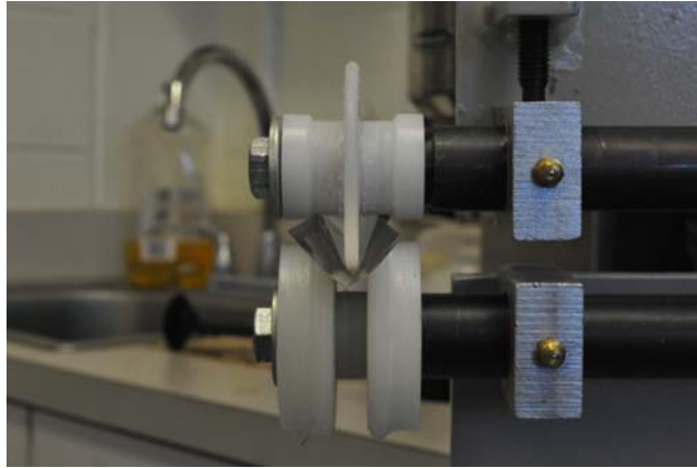
Figure 2: Bead Roller Geometry
