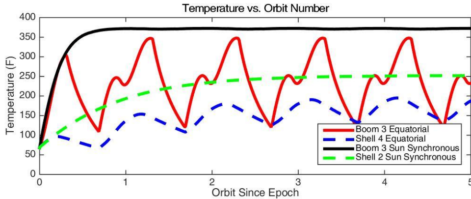
Figure 19: On-Orbit Temperatures Estimated via Numerical Simulations
