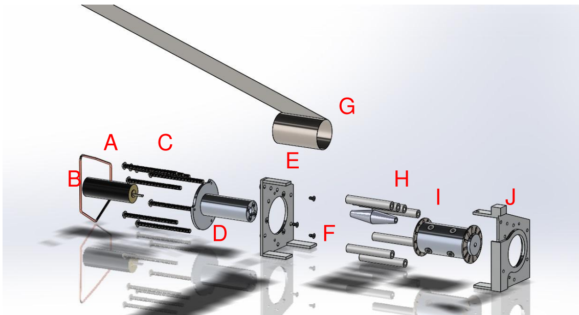
Figure 7: Assembly of a Single Deployer
