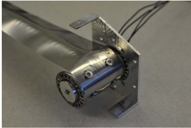
Figure 5: Drum is Placed Over Sleeve
