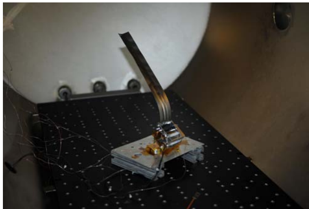
Figure 25: Boom Curved Unexpectedly in Thermal Vacuum Chamber
