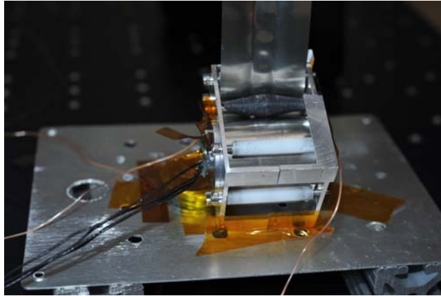
Figure 24: Thermocouple Locations
